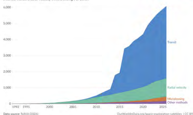
Cumulative number of exoplanets discovered, by method
